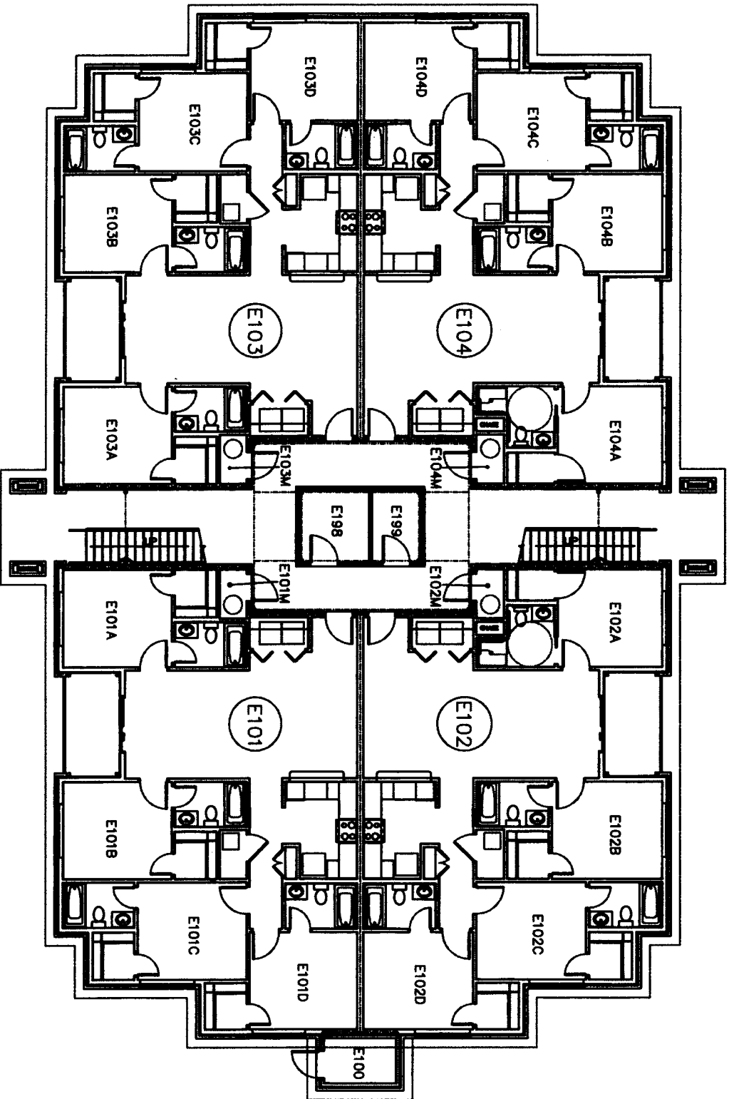
Building "E" - First Floor Plan
