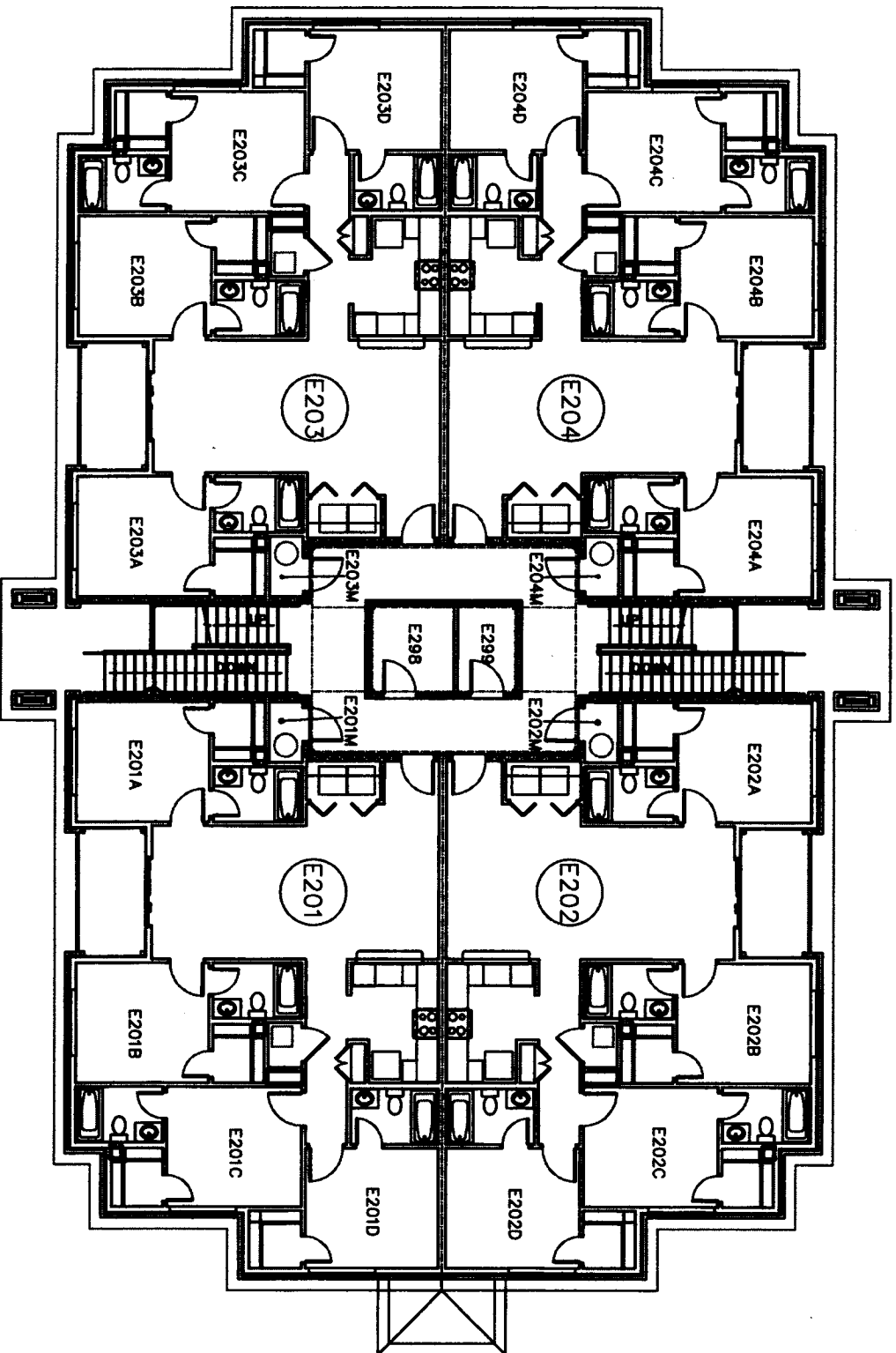
Building "E" - Second Floor Plan
