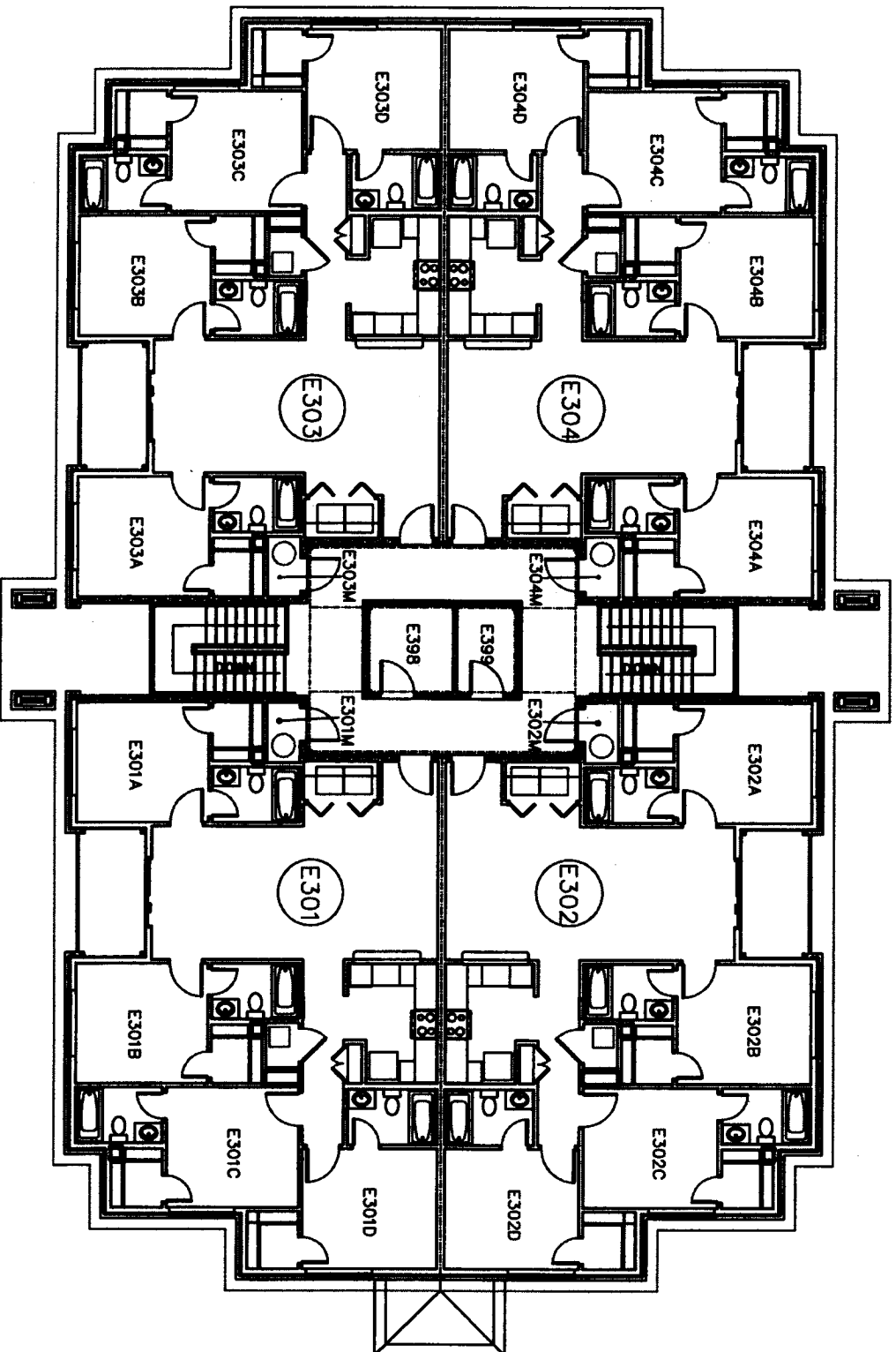
Building "E" - Third Floor Plan
